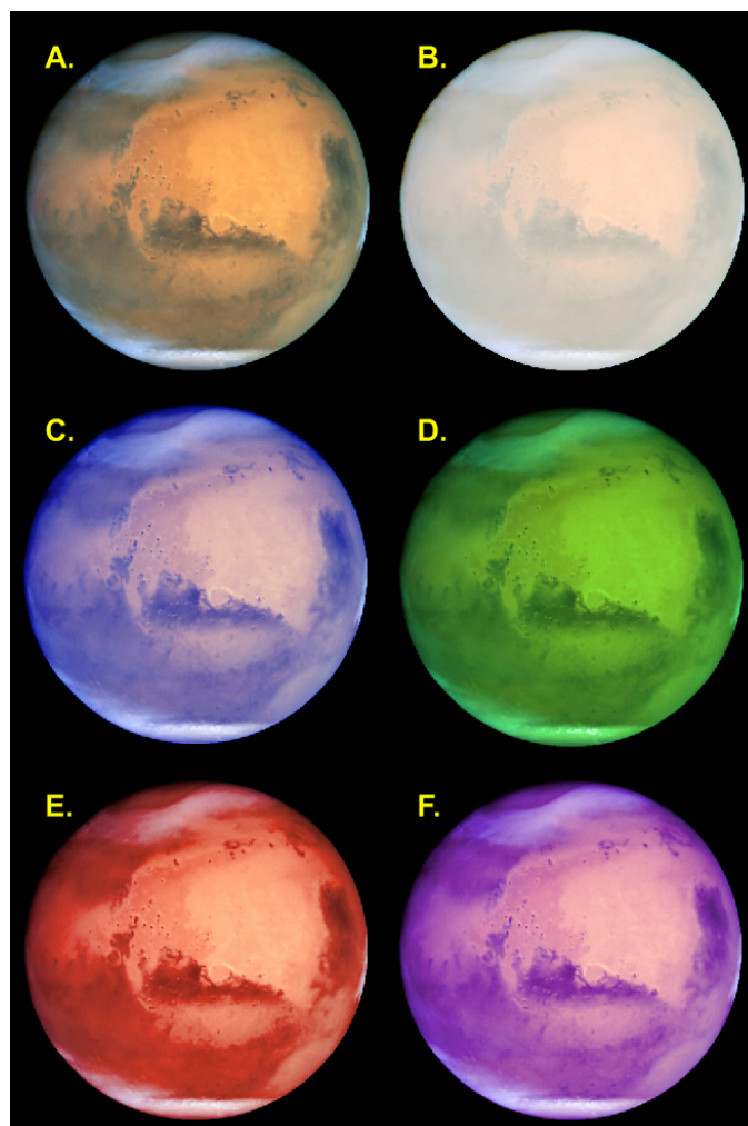
Figure 2. How Filter Colours Affect A Planet's Appearance: In this computer simulation, the effect of colour filters on the appearance of Mars is shown. A. is the natural appearance of the planet as observed from space; B. is how the planet generally looks through an amateur telescope; C. is with a blue filter applied, highlighting clouds and polar caps as well as improving contrast, D. is with a green filter, doing little to improve the view; E. is with a red filter, greatly increasing contrast but cutting out clouds and polar caps; and F. is with a magenta filter, combining the benefits of both a blue and red filter. Original Mars image from HST.
